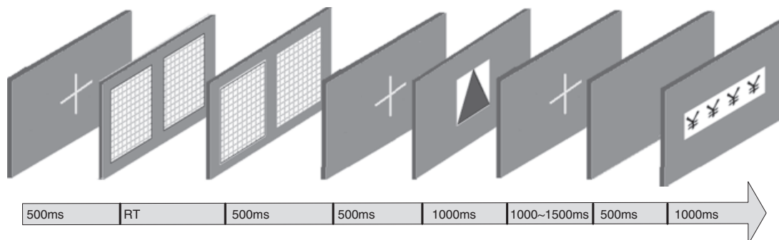
Figure 2. Sequence and durations of stimuli and events in each trial.
